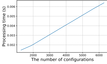
Fig. 5. Processing time of SC-DCRC with increasing number of configurations.
