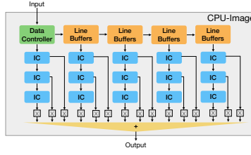
Fig. 10. The CPU-image implementation.
