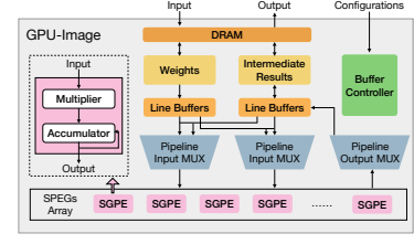
Fig. 11. The GPU-image implementation.
